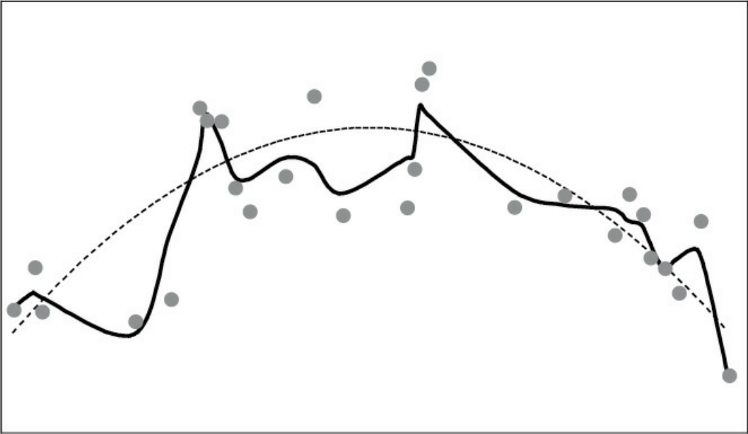
FIGURE 5-6C: OVERFIT MODEL
