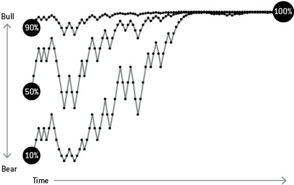
FIGURE 8-8: BAYESIAN CONVERGENCE
